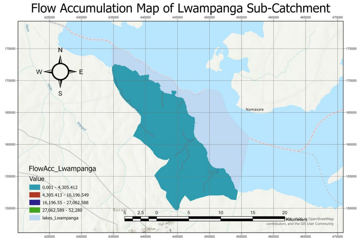
Figure 3: Flow Accumulation, Drainage channels
